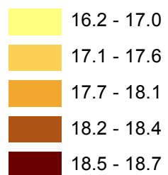
WSAVG - average temperature across the 2006 summer period (May 26th-August 31st)
